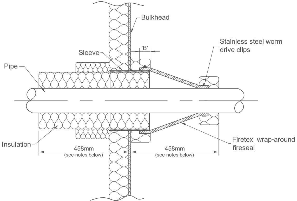
(SECTIONAL VIEW)
