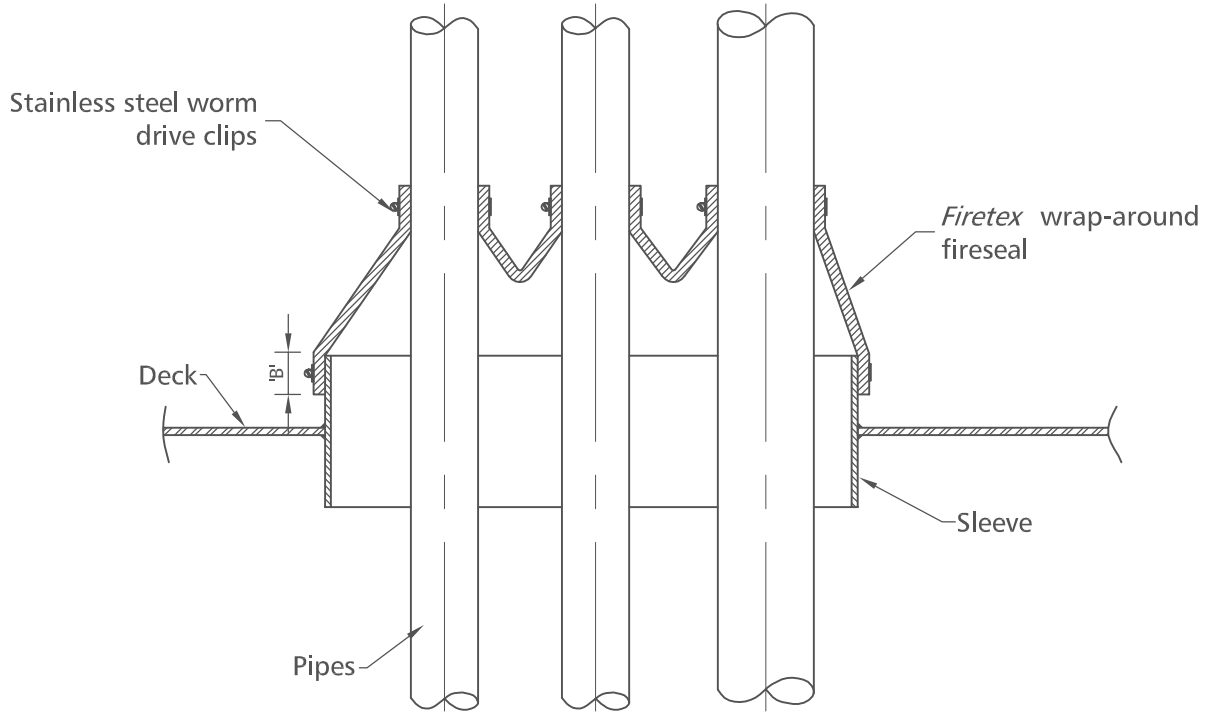
(SECTIONAL VIEW)
