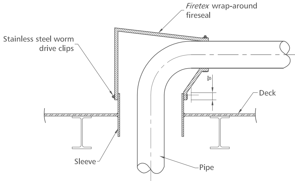
(SECTIONAL VIEW)
